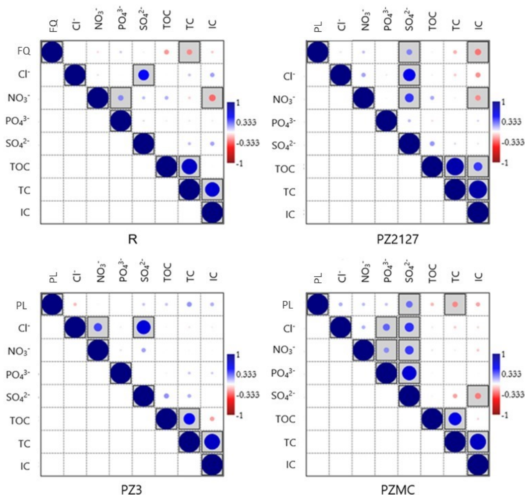
Figure 5 – Pearson correlation coefficients ( \rho ) between fluvimetric quota (FQ), phreatic level (PL), and chemical species concentrations in the river and piezometer water.
